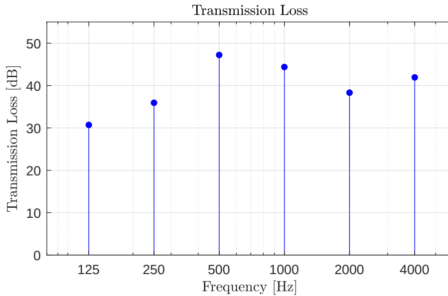
Figure 5: Transmission loss per octave band.
